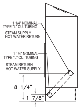
TWO ROW COIL PIPING DIMENSIONS.
